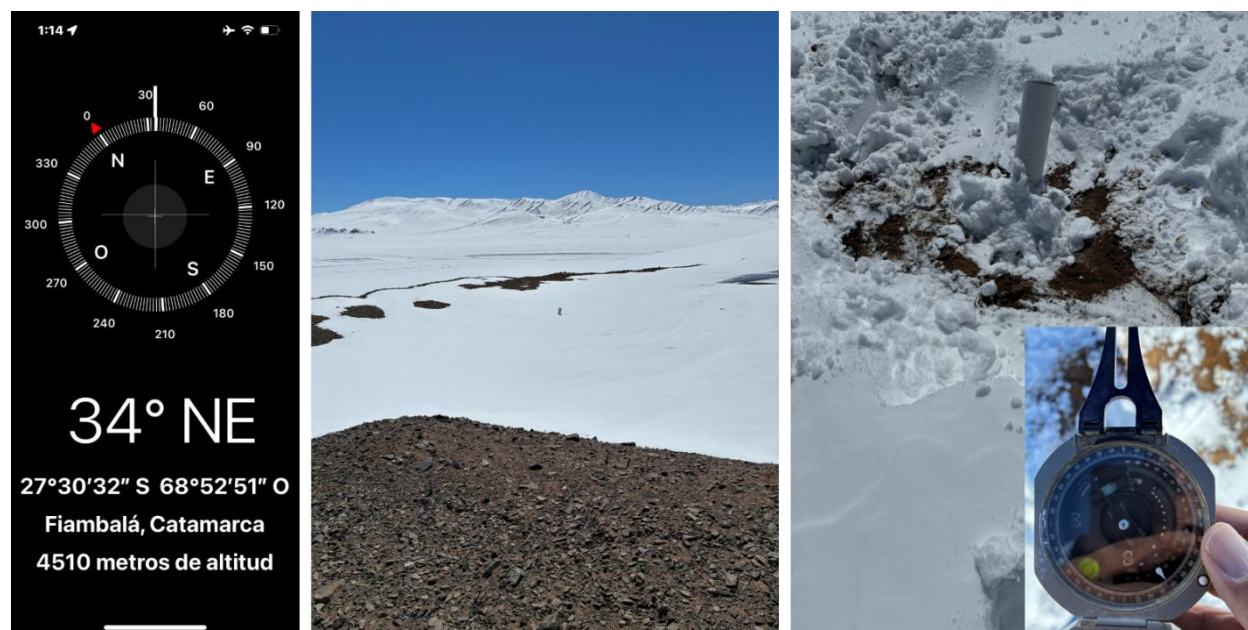
Figure 12-5: Point 1, Drill Hole LVR49
