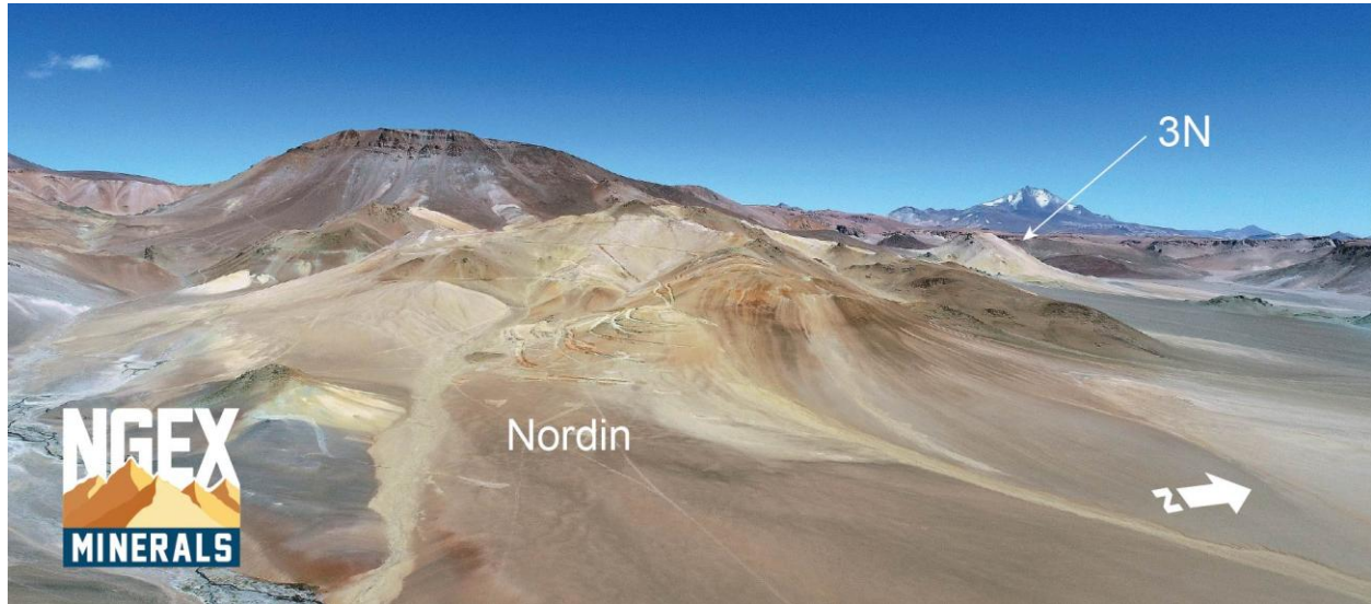
Figure 7-3: View to the Northwest over the Nordin Target
