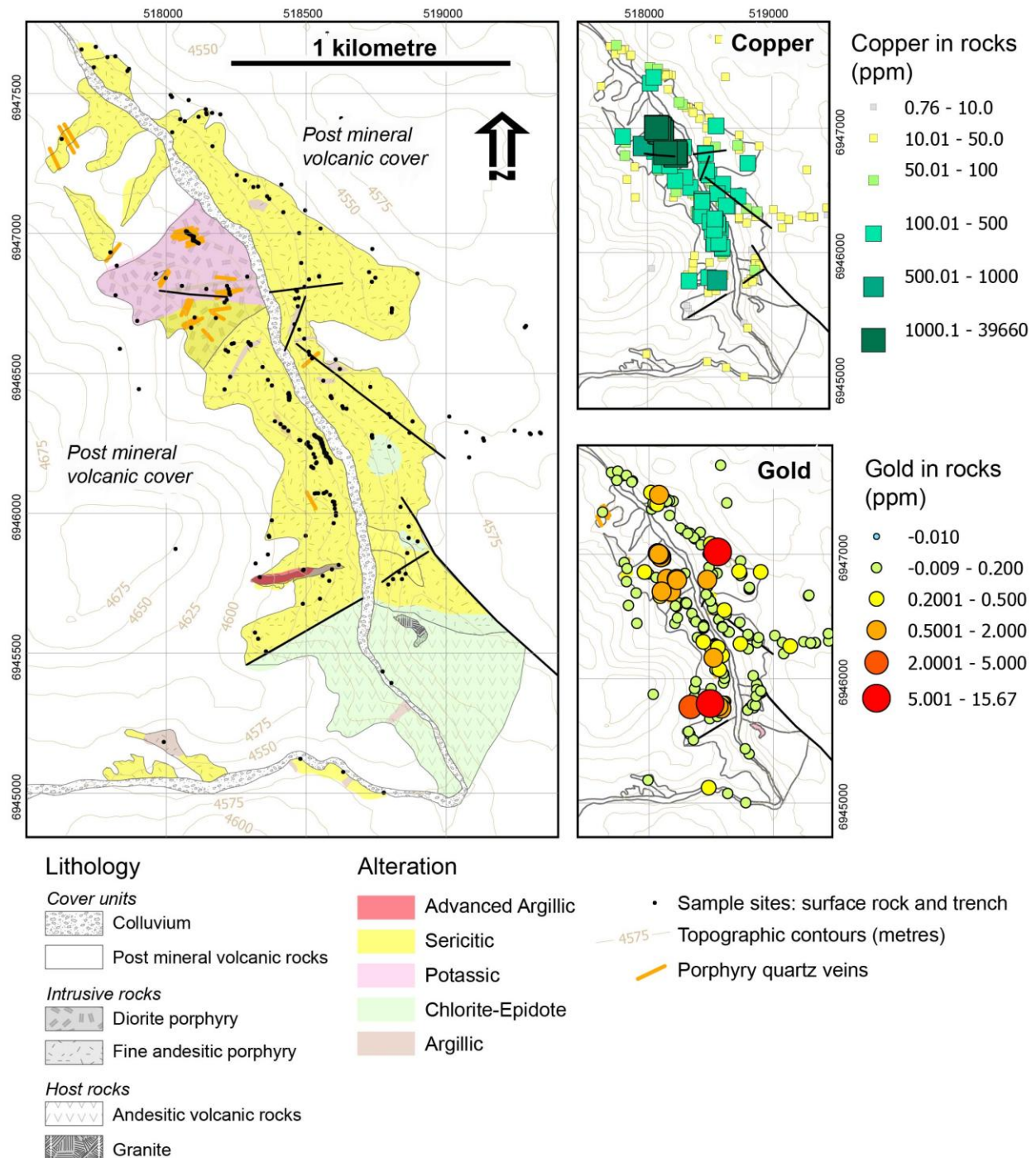
Figure 7-8: Geology of the La Quebrada Target
