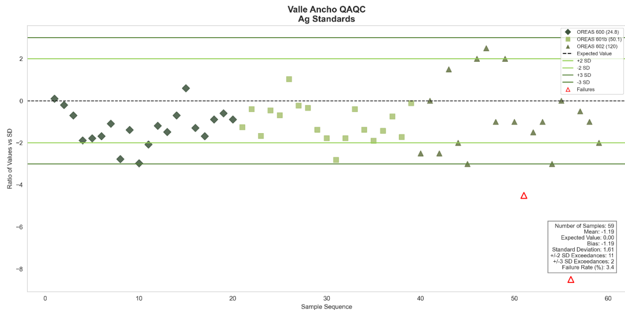
Figure 11-3 CRMs OREAS 600, OREAS 601b, and OREAS 602, Showing Low, Medium and High Ag ppm Grades
