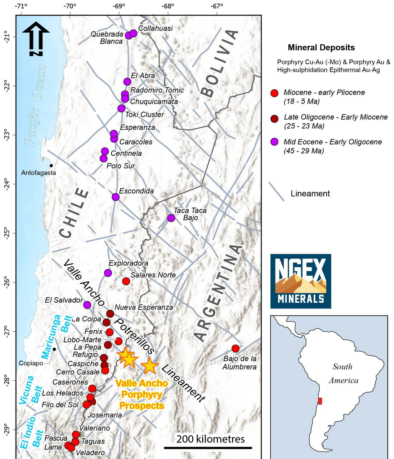
Figure 7-1: Eocene to Miocene Porphyry and High-sulphidation Epithermal Deposits, Central Andes
