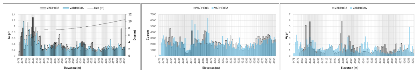
Figure 12-8: DDH VADH003 vs VADH003A
