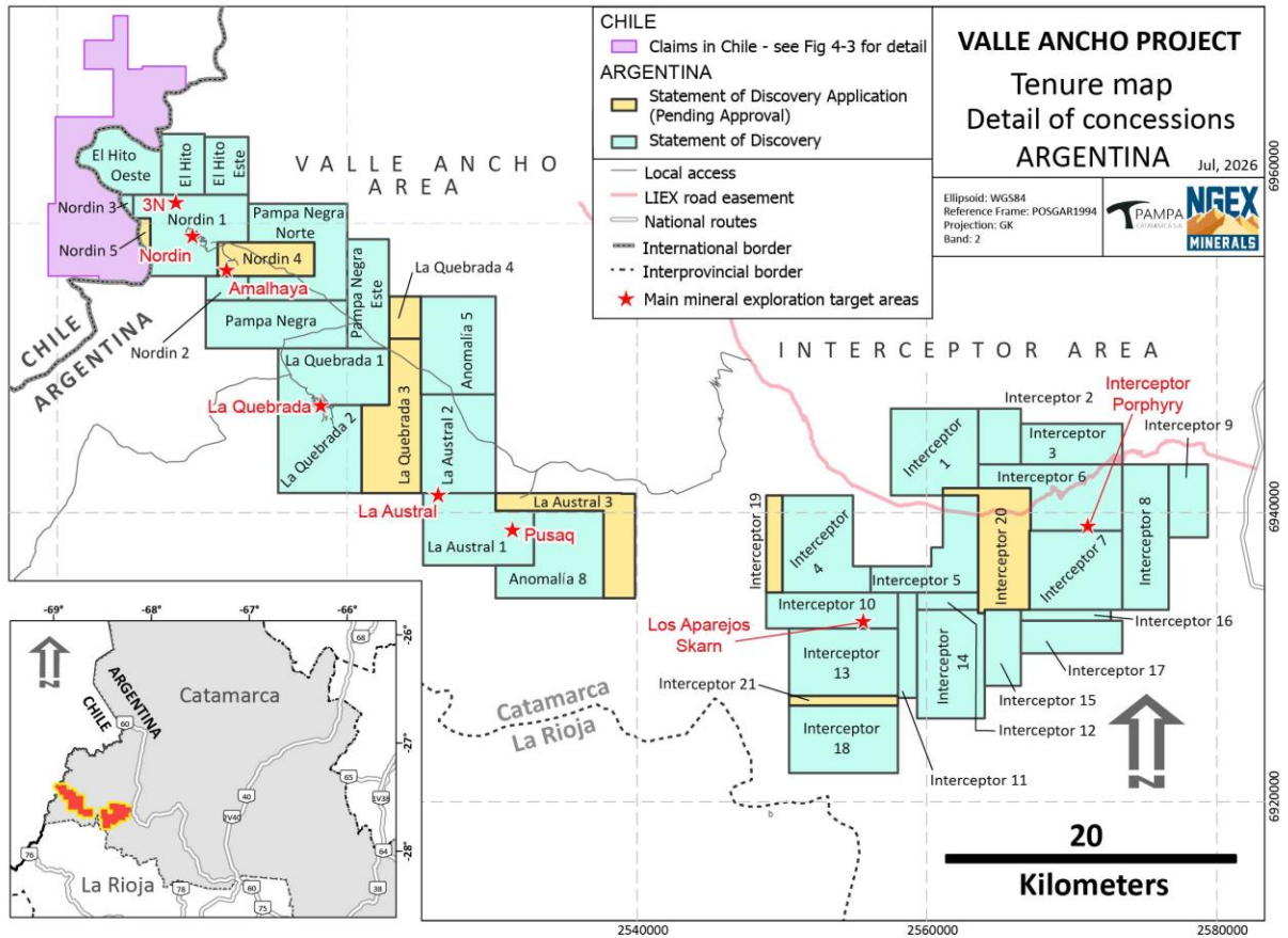
Figure 4-2: Mineral Tenure Map Argentina
