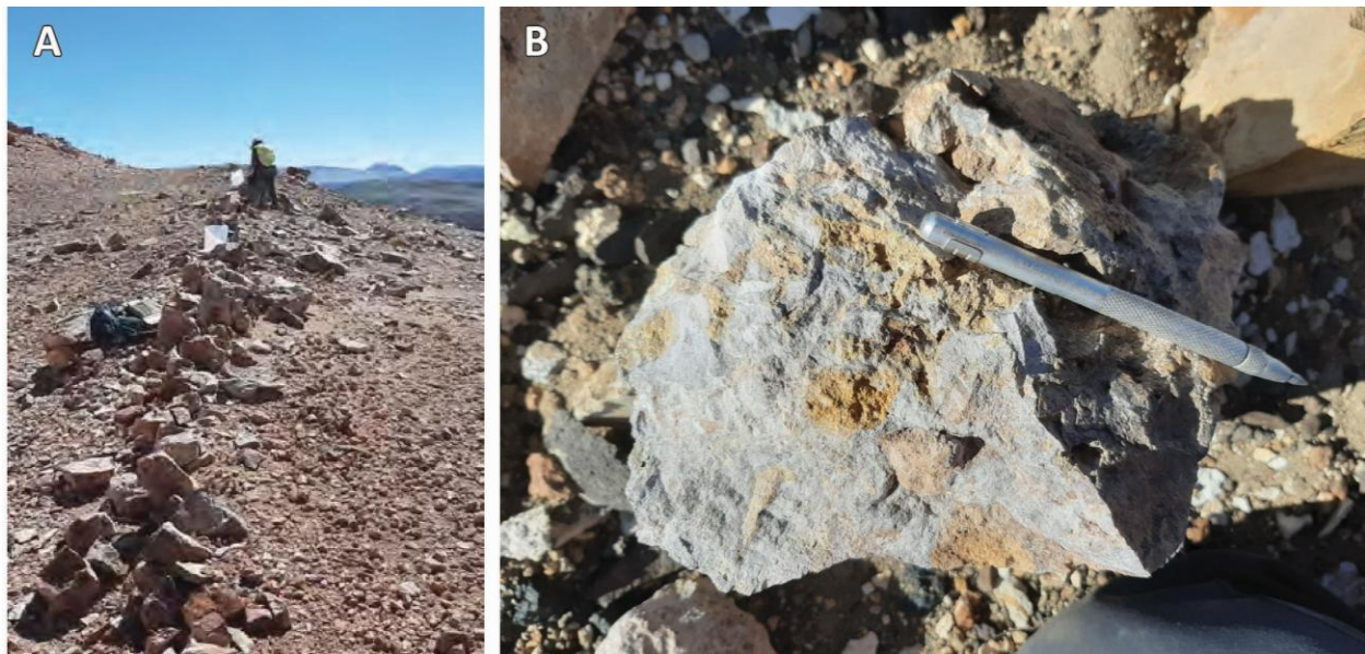
Figure 7-9: Outcrop Photos from La Austral
