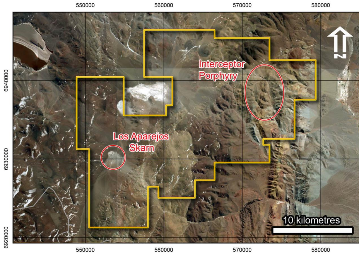
Figure 9-2: Exploration Targets in the Interceptor Area
