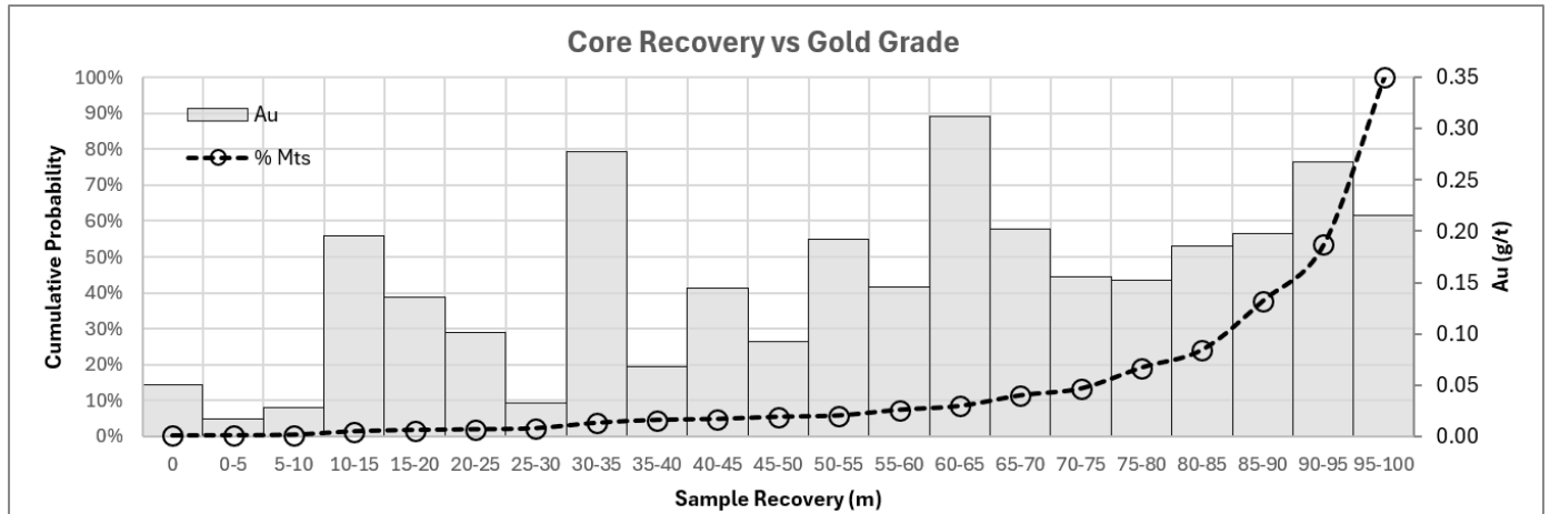
Figure 10-2: Core Recovery vs. Gold Grade
