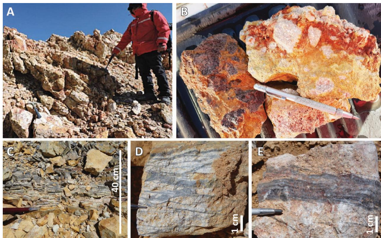
Figure 7-5: Photos of Hydrothermal Breccias at Nordin
