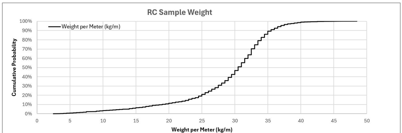
Figure 10-3: RC Sample Weight
