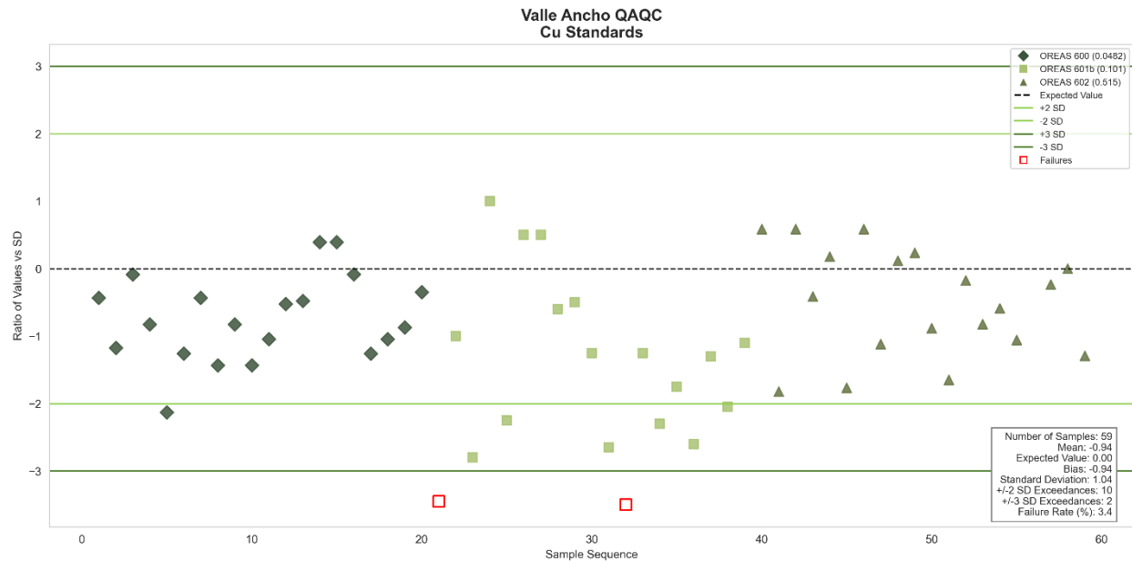
Figure 11-2 CRMs OREAS 600, OREAS 601b, and OREAS 602, Showing Low, Medium, and High Cu % Grades
