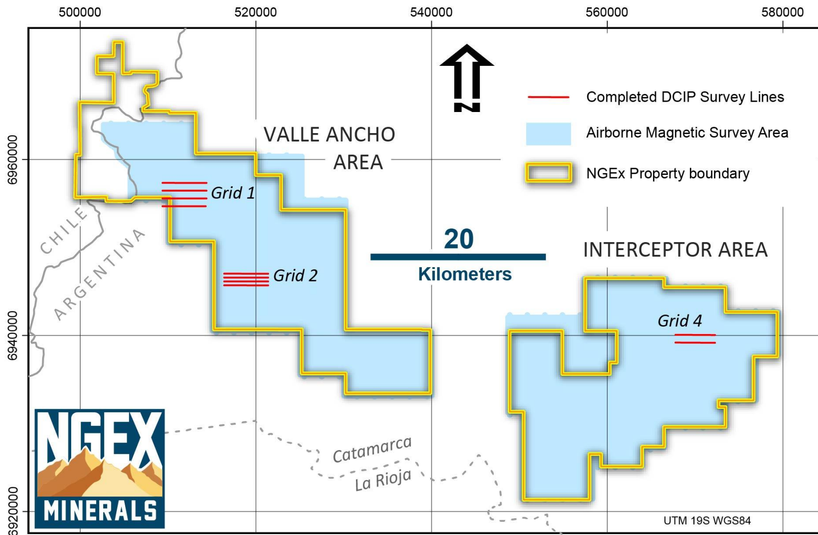
Figure 9-9: IP/Resistivity Grid Locations in the Valle Ancho and Interceptor Areas
