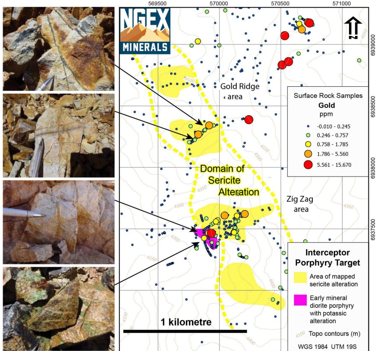
Figure 7-10: Alteration and Mineralization Features at the Interceptor Porphyry Target
