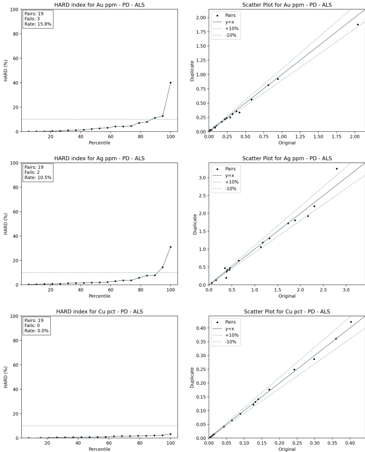
Figure 11-9: Pulp Duplicate Plots for Au ppm, Ag ppm and Cu pct
